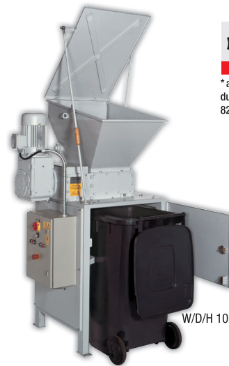
intimus VZ Spezial S 28/35 | M 35/35 W/D/H 102 x 103/175 x 189/245 cm with open doors / folded up hopper lid
